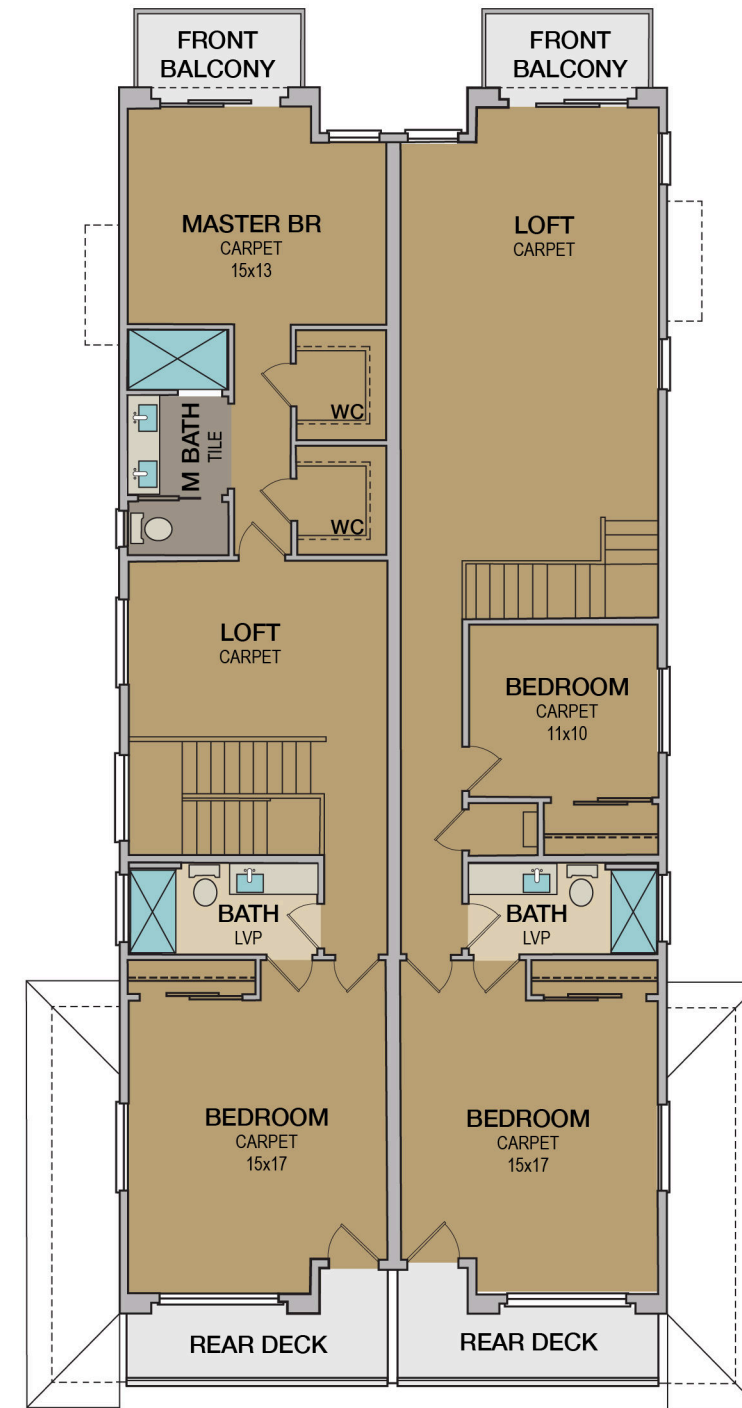
FLOOR PLAN A
