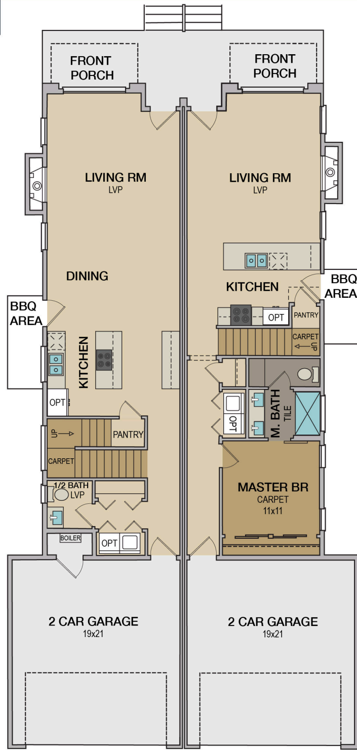
FLOOR PLAN A
